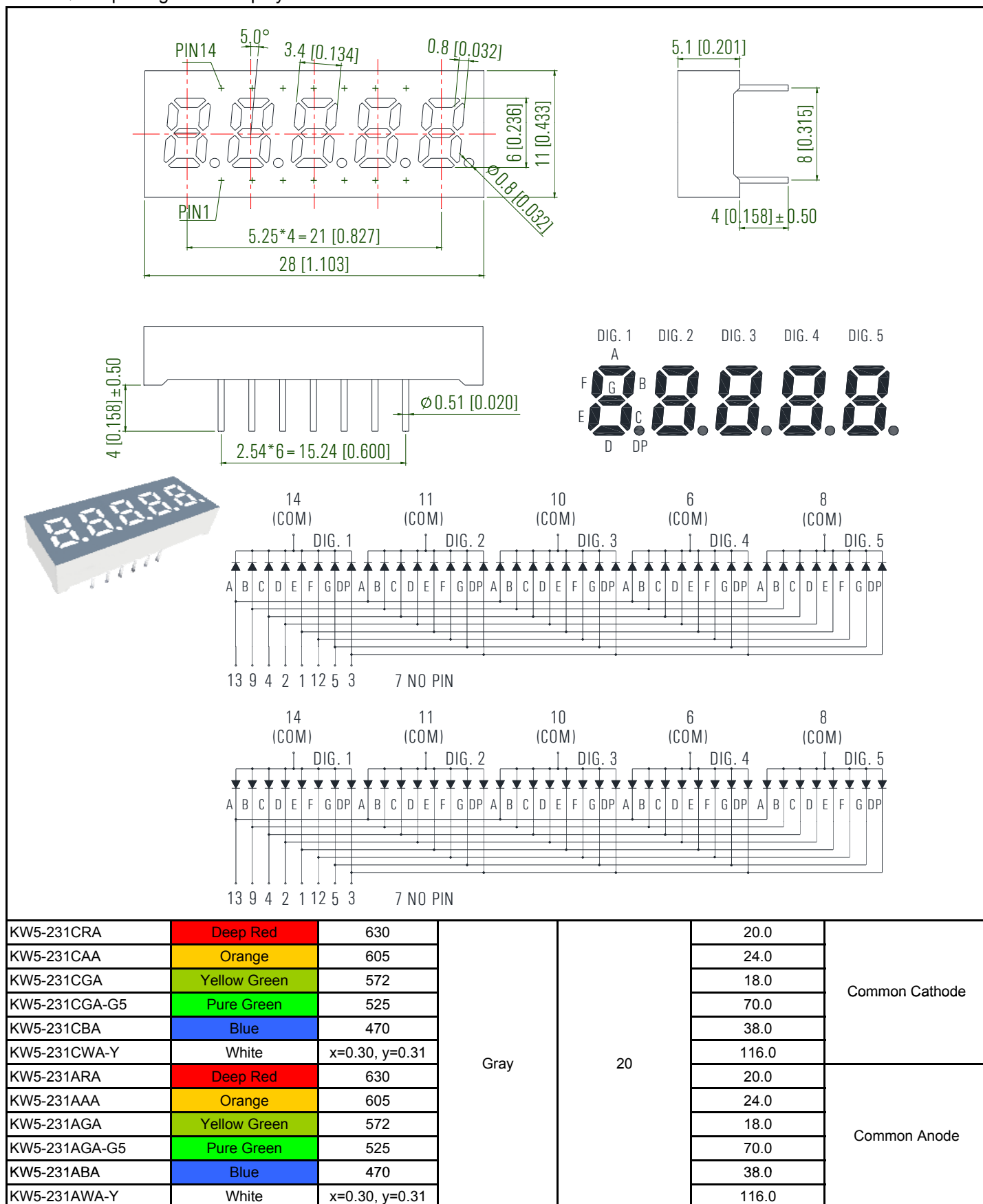
0.23" Quintuple Digit LED Display
