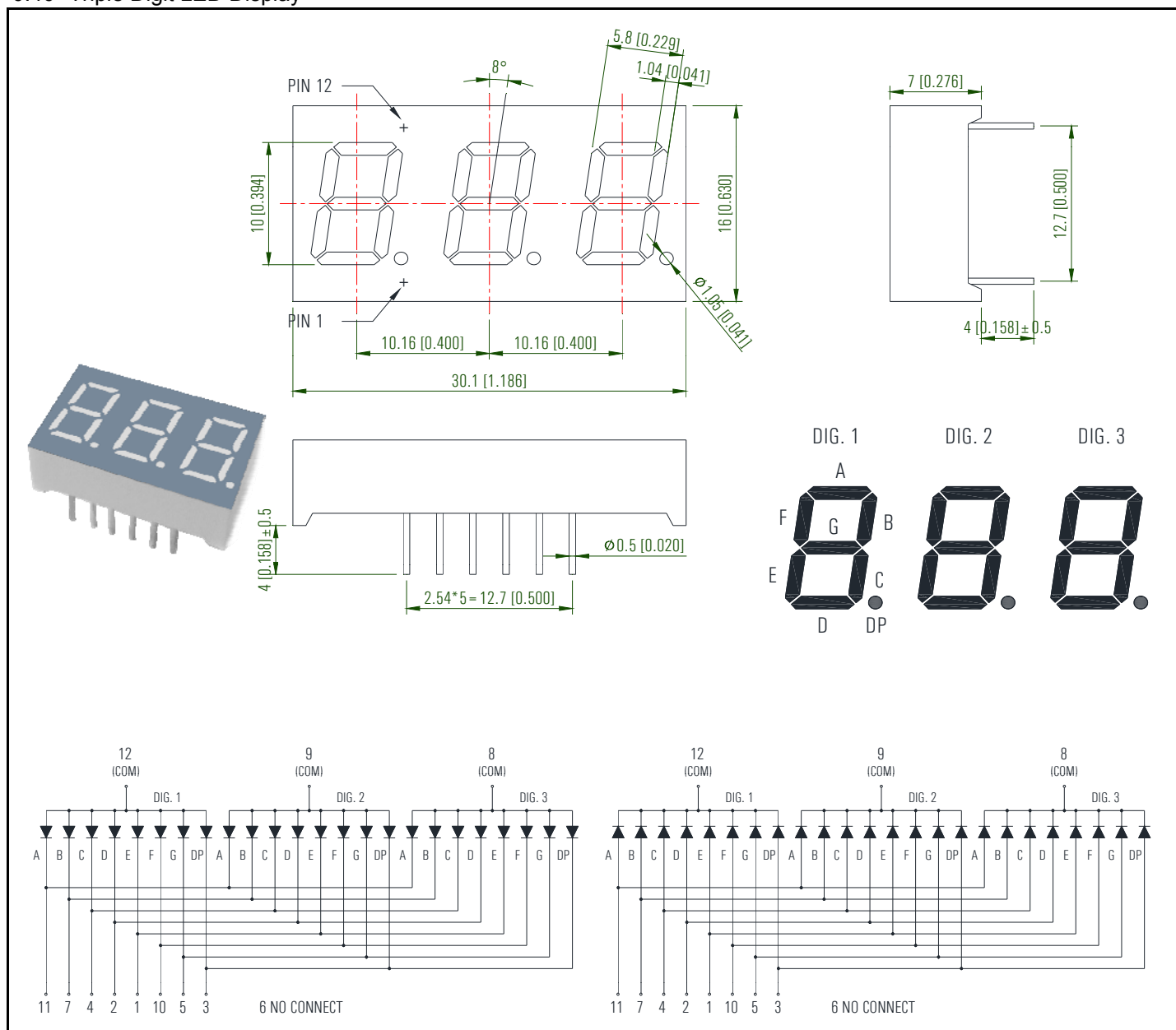
0.40" Triple Digit LED Display
