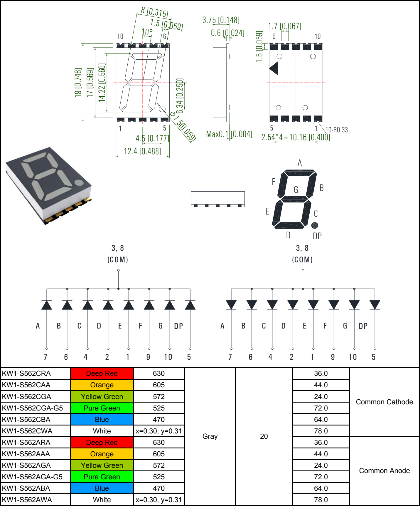
0.56" Single Digit SMD Display
