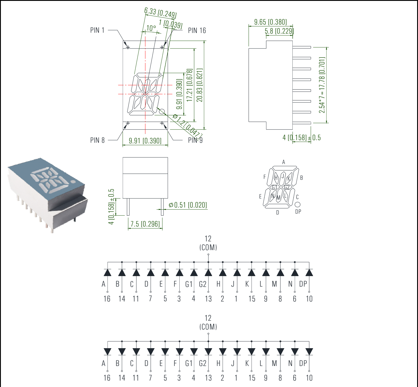
9.90mm (0.39inch) Single Digit Alphanumeric LED Display
