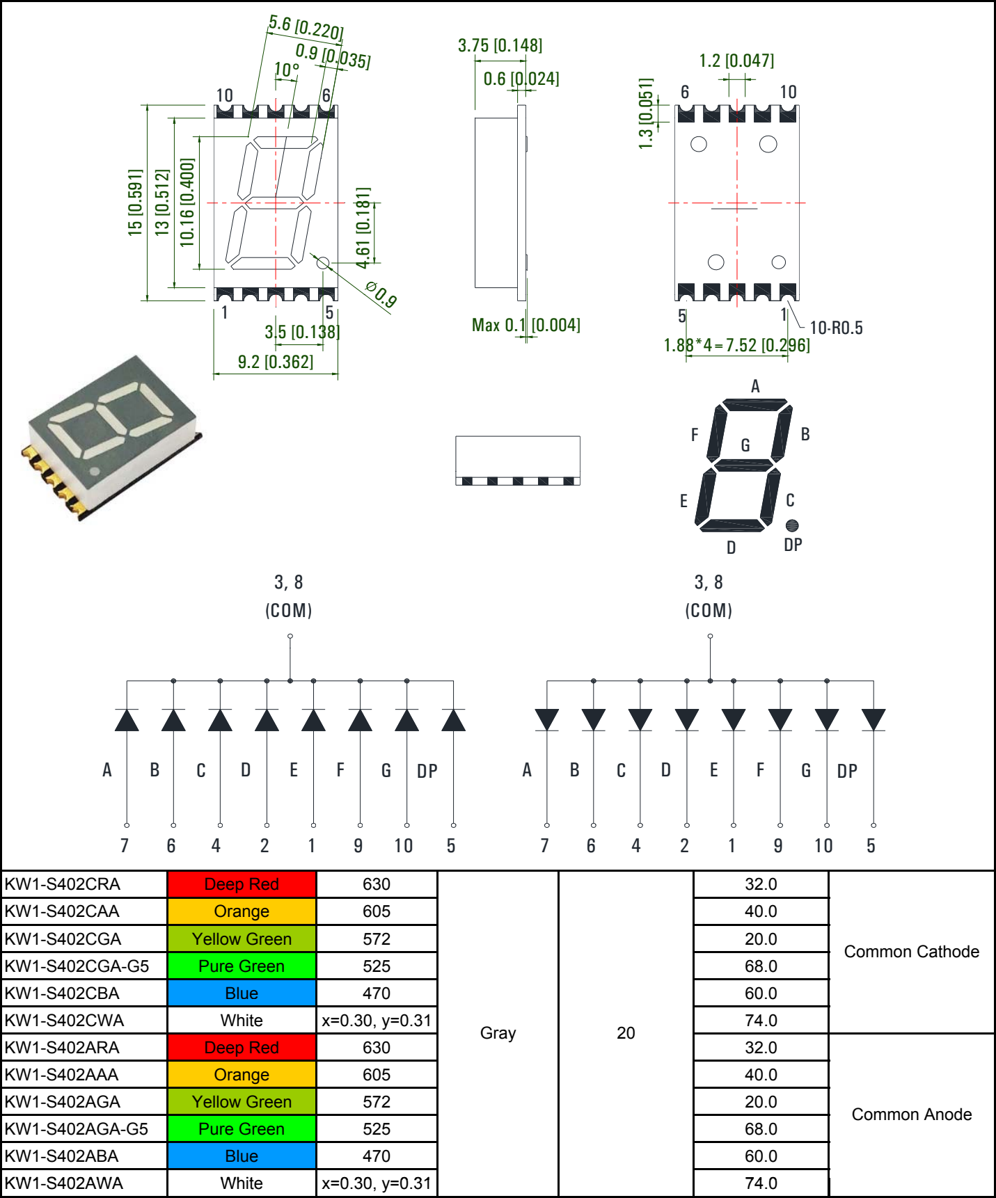
0.40" Single Digit SMD Display
