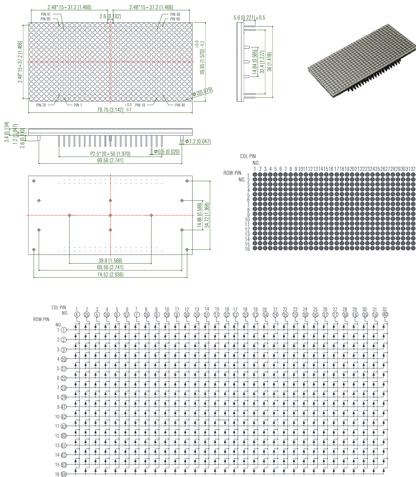
3.1" 32×16 Single Color Dot Matrix
