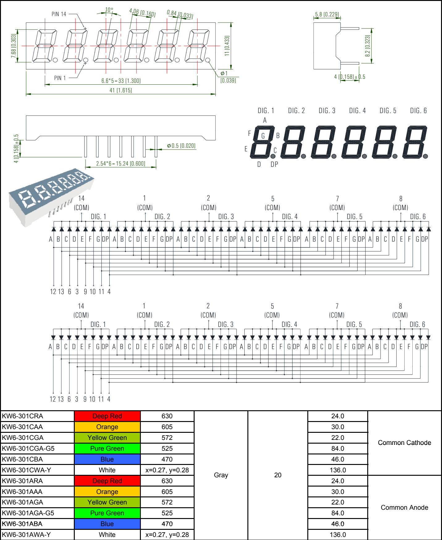
0.30" Six Digit LED Display
