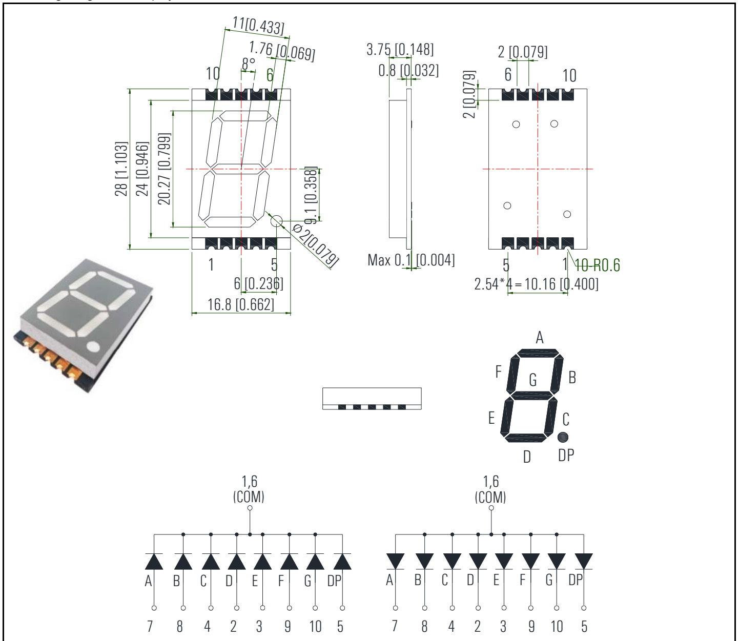
0.80" Single Digit SMD Display
