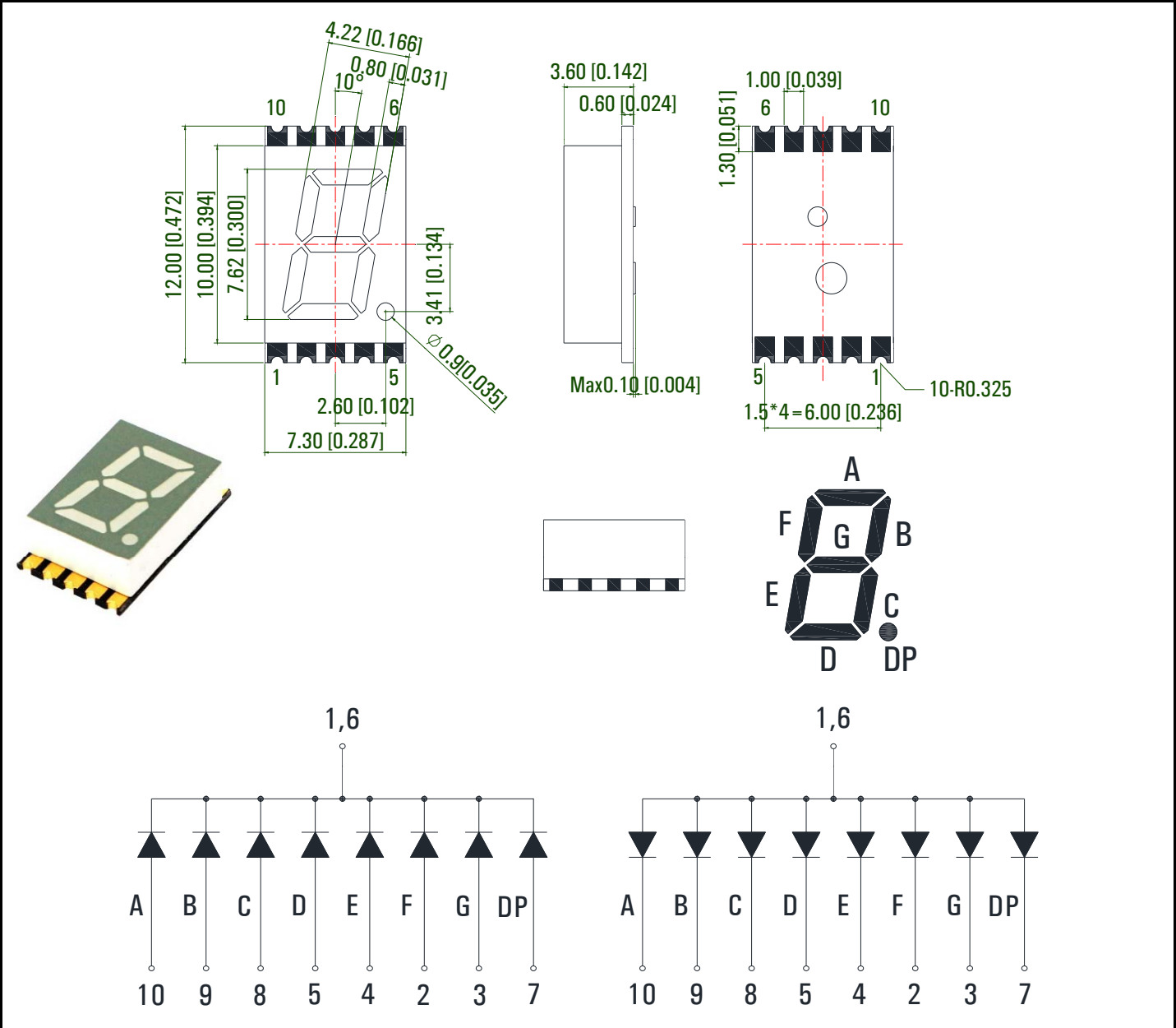
0.30" Single Digit SMD Display
