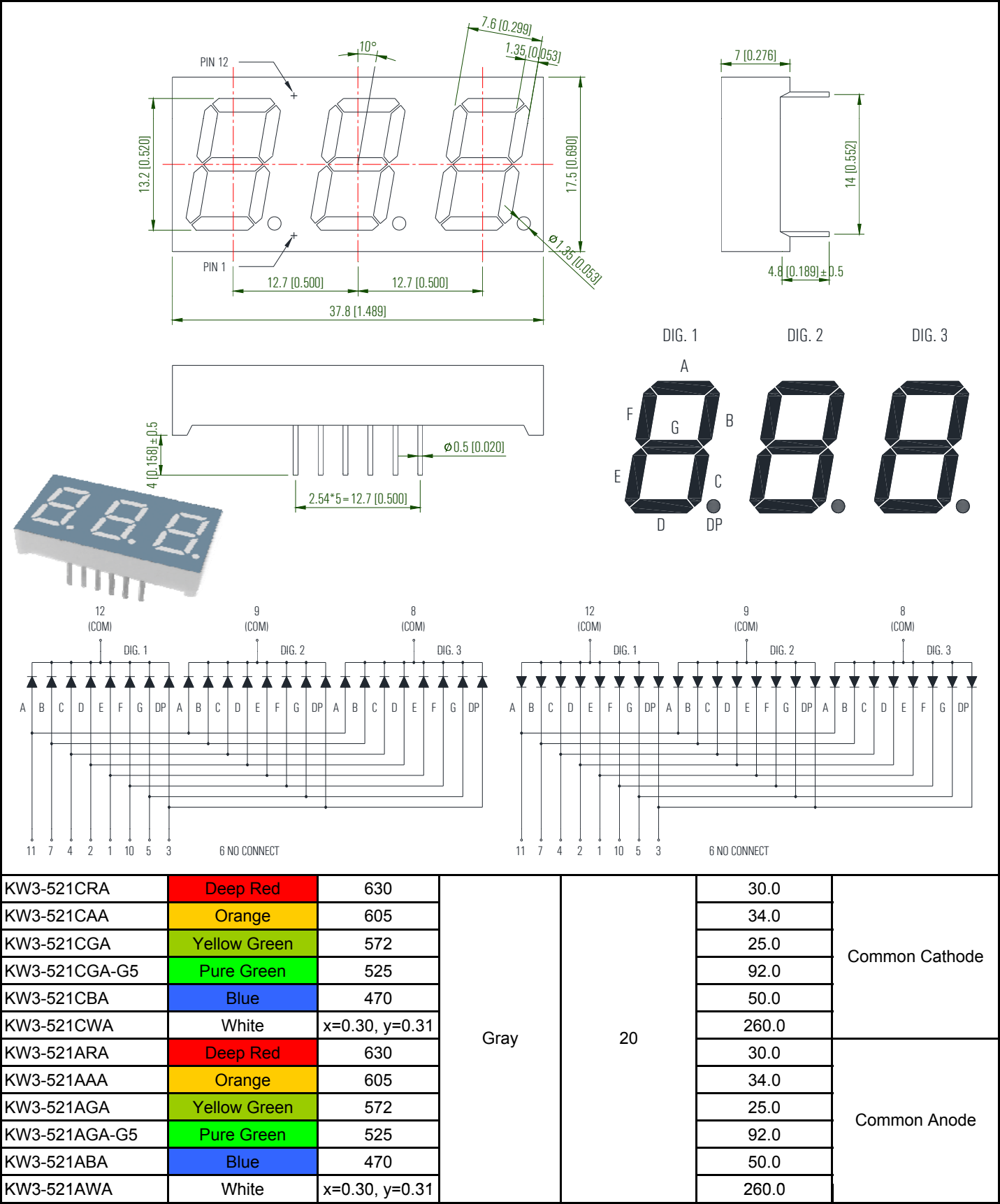
0.52" Triple Digit LED Display
