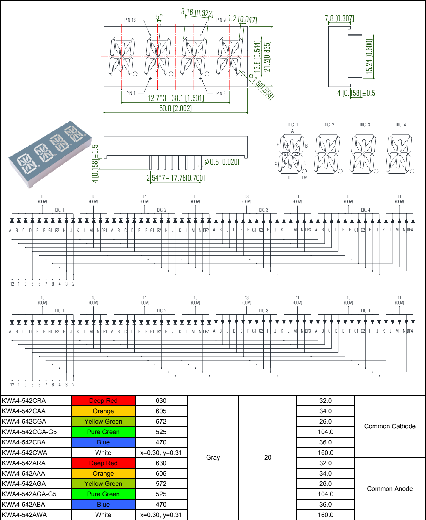
13.80mm (0.54inch) Quadruple Digit Alphanumeric LED Display
