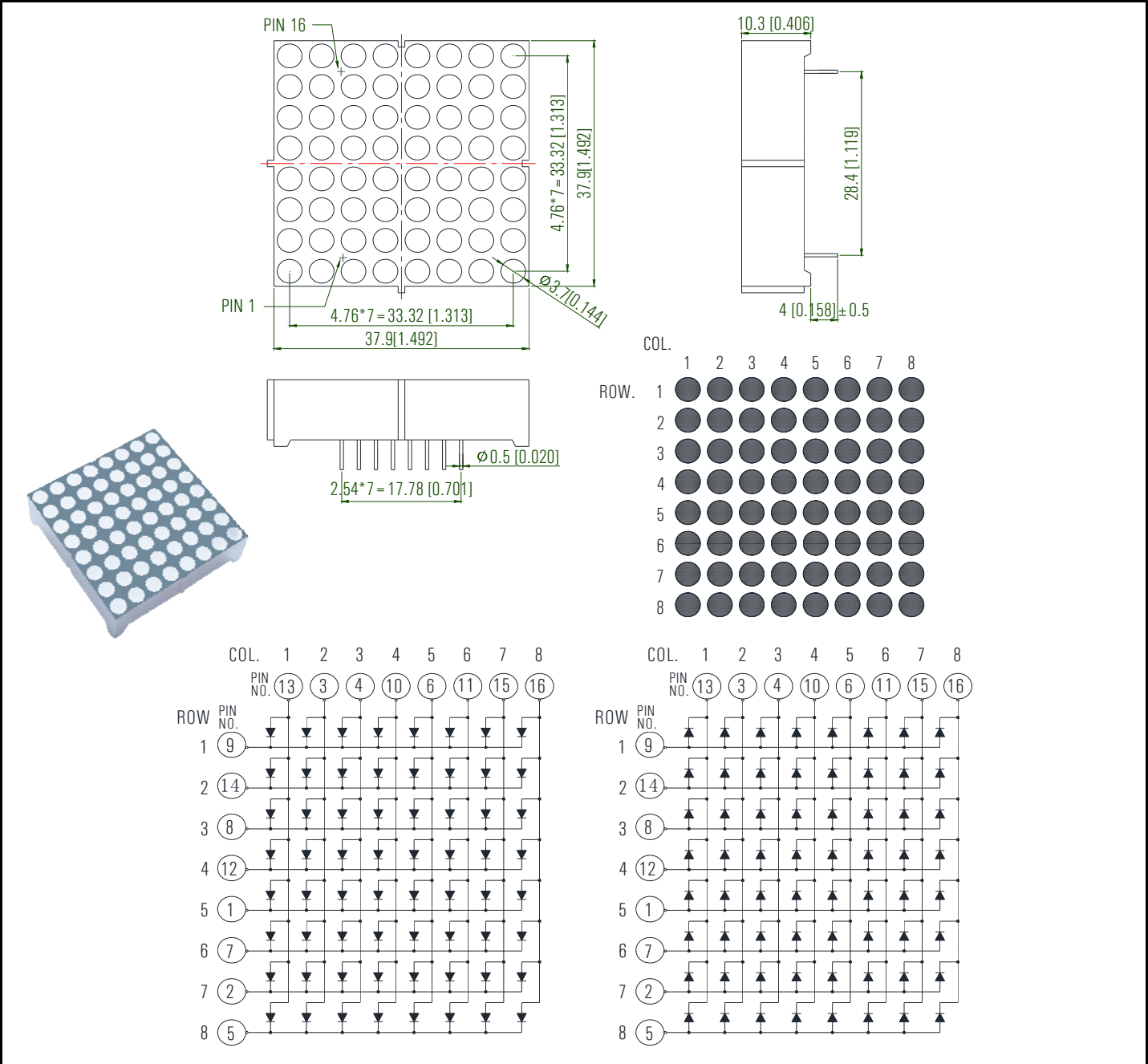
1.5" 8×8 Single Color Dot Matrix
