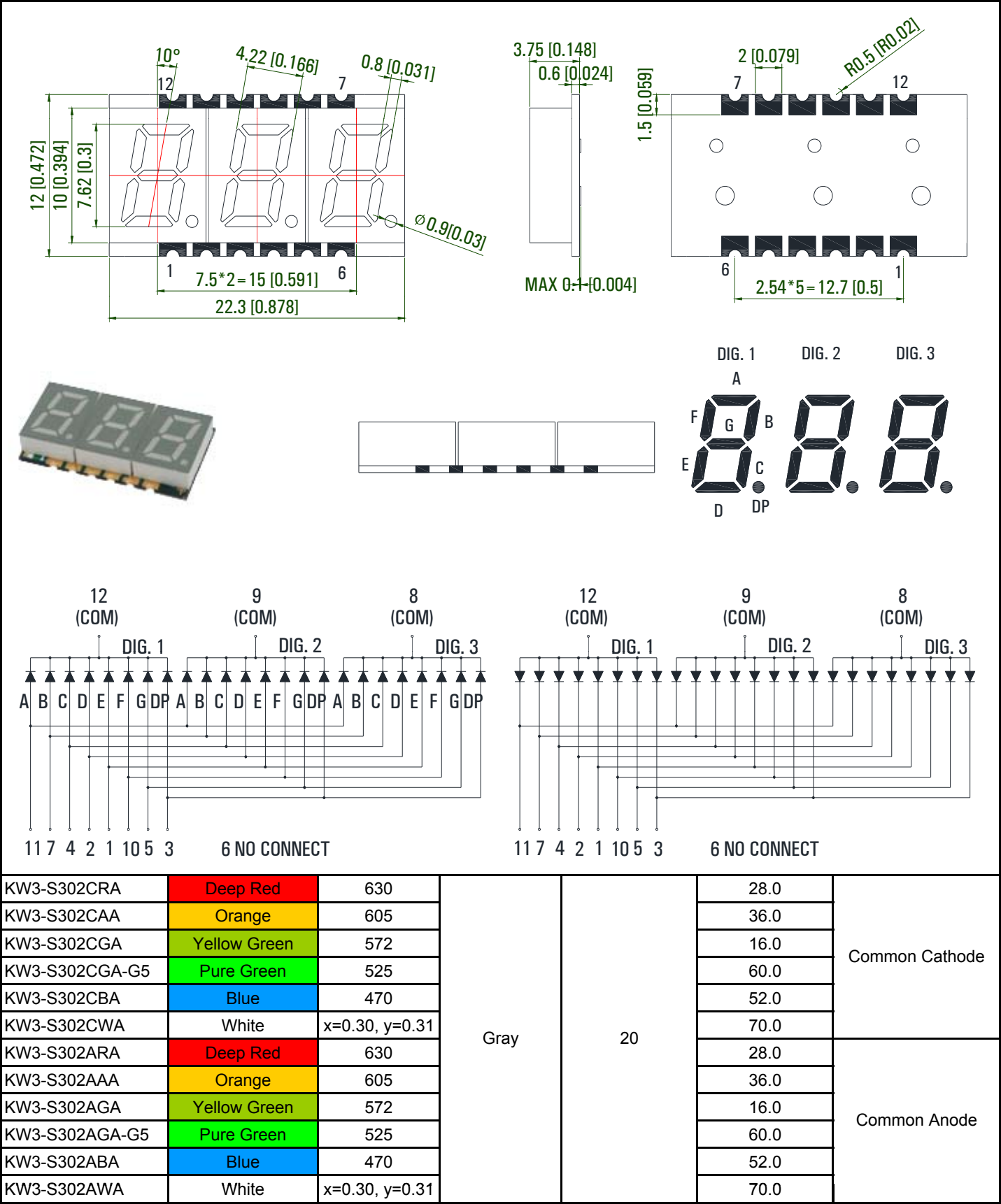
0.30" Triple Digit SMD Display
