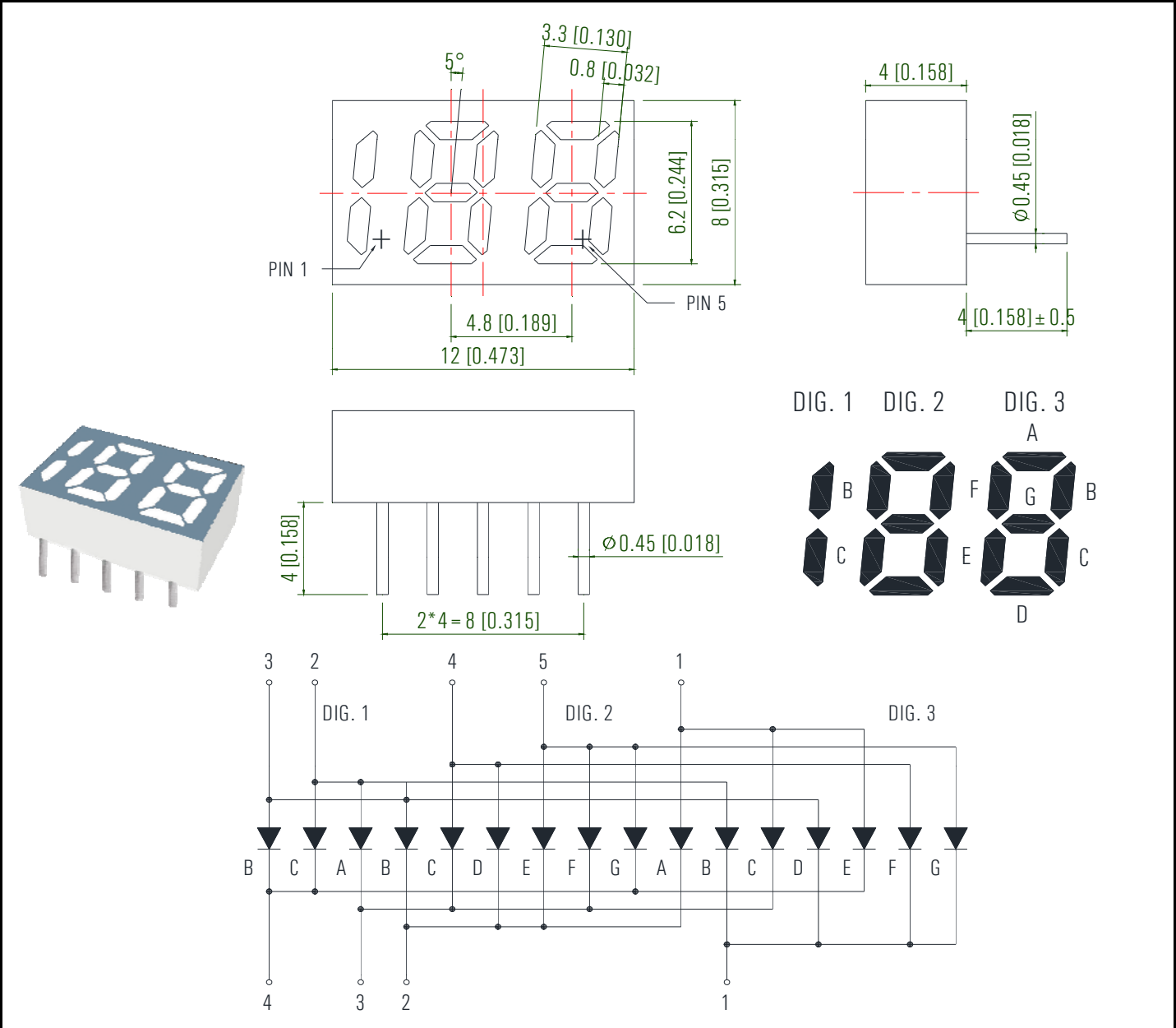
0.25" Dual Half Digit LED Display
