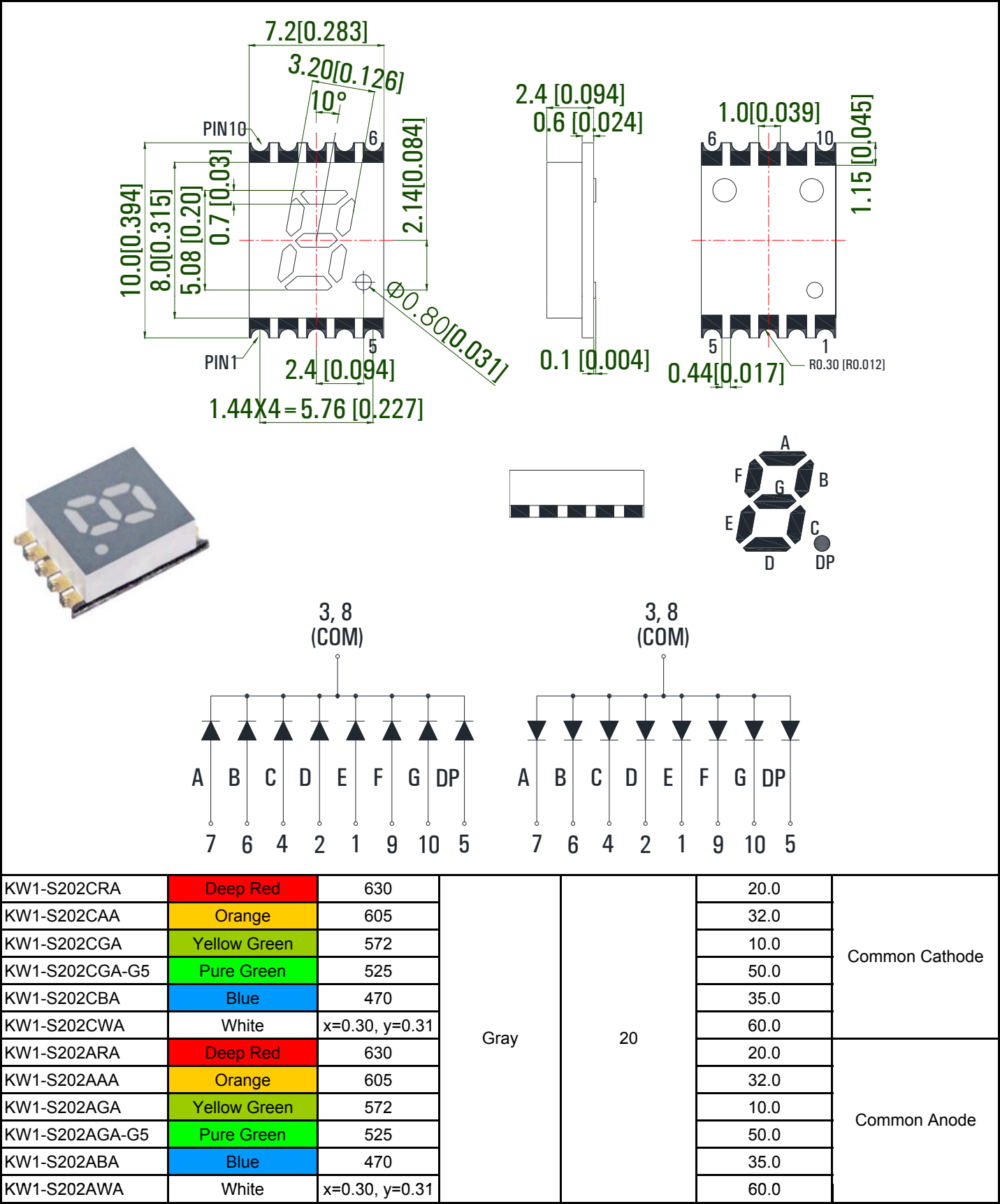
0.20" Single Digit SMD Display
