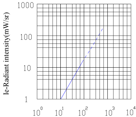
IF-Forward Current(mA)
