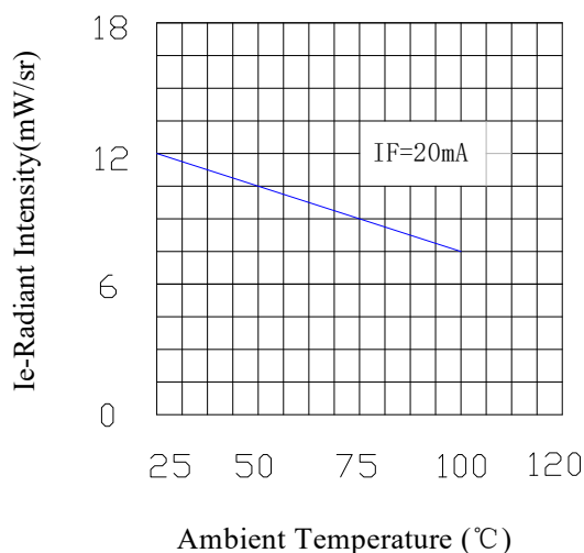
Relative Intensity & Ambient Temperature(°C)
