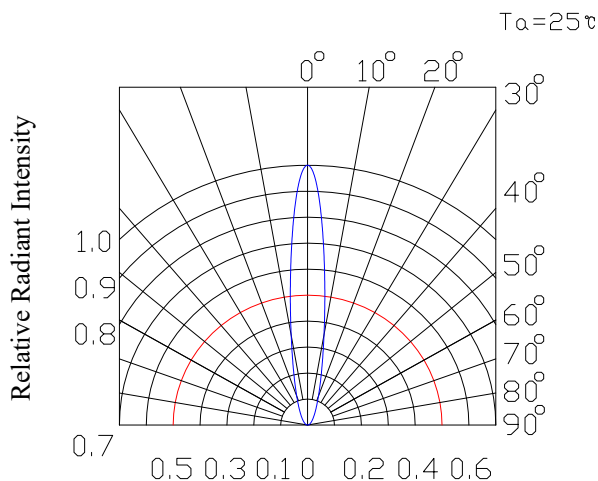
Relative Radiant Intensity & Angular Displacement
