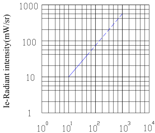
IF-Forward Current(mA)
