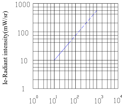
IF-Forward Current(mA)
