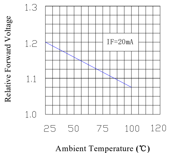
Forward Voltage & Ambient Temperature(°C)
