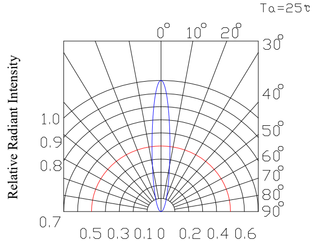
Relative Radiant Intensity & Angular Displacement
