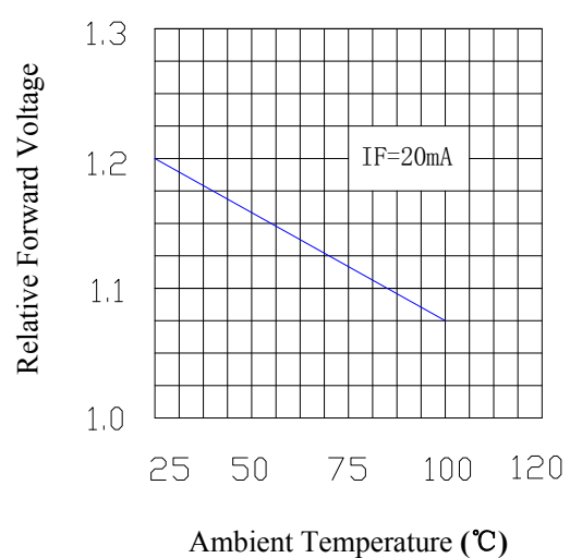
Forward Voltage & Ambient Temperature(°C)
