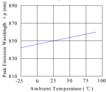
Peak Emission Wavelength & Ambient Temperature
