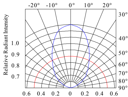
Relative Radiant Intensity & Angular Displacement
