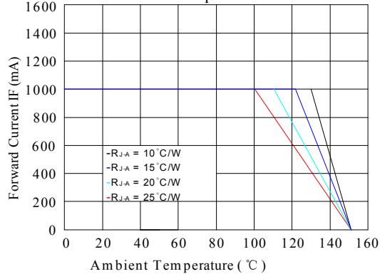
Maximum Forward Current & Ambient Temperature
