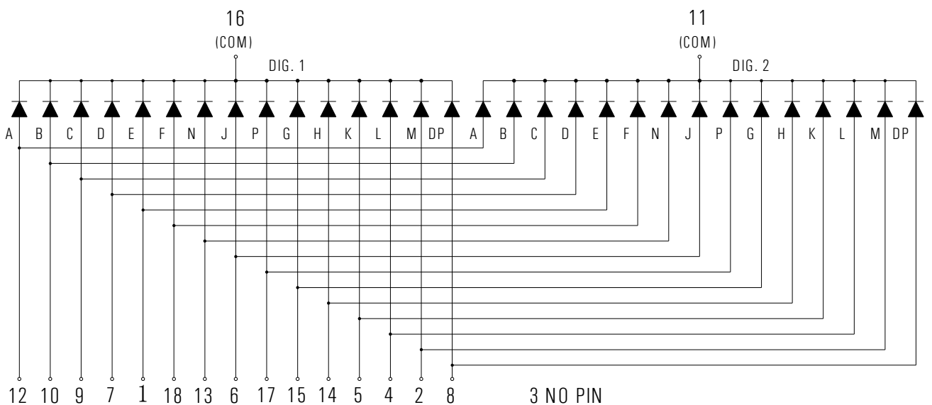
KA2-541CBB (Common Cathode)
