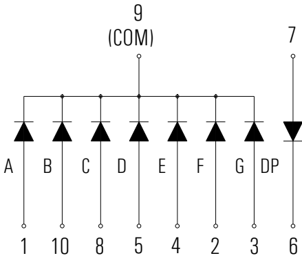
KD1-321CRD (Common Cathode)
