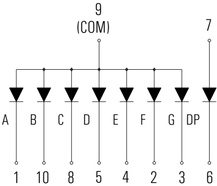
KD1-321ARD (Common Anode)
