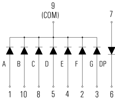
KD1-321CYD-2B (Common Cathode)
