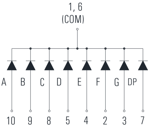
KD1-40NCYD-2B (Common Cathode)
