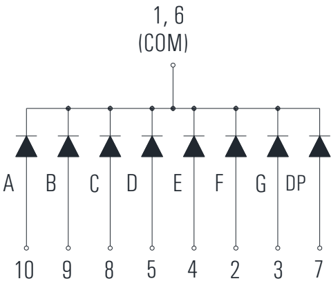
KD1-40NCYD-3C (Common Cathode)
