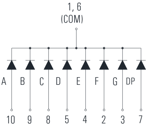
KD1-40NCGD-2B (Common Cathode)
