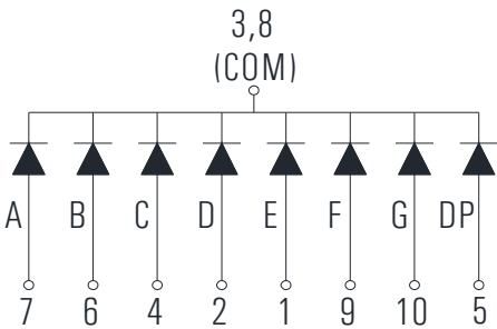
KD1-571CGD-2B (Common Cathode)
