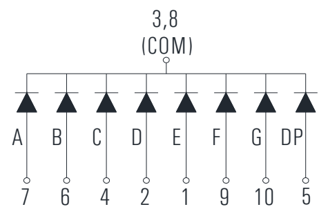
KD1-571CYD-2B (Common Cathode)
