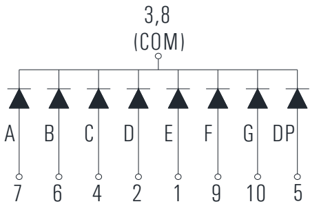
KD1-571CYD-3C (Common Cathode)
