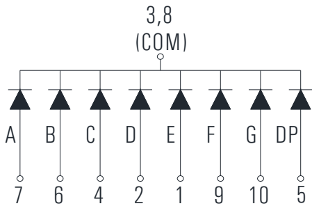
KD1-571CAD-2B (Common Cathode)
