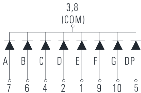
KD1-571CVD-2B (Common Cathode)
