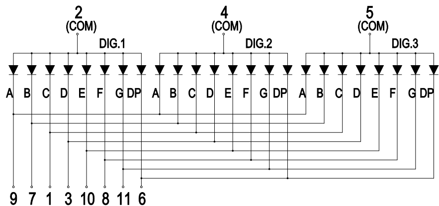
KD3-307AGD (Common Anode)
