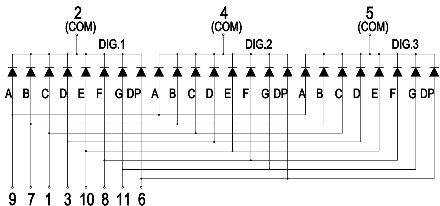
KD3-307CGD (Common Cathode)
