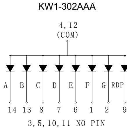
Internal Circuit Diagram (Common Anode)
