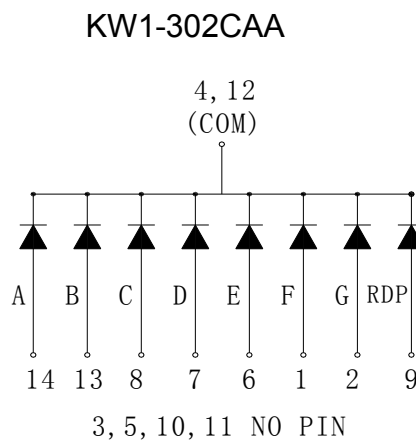
Internal Circuit Diagram (Common Cathode)
