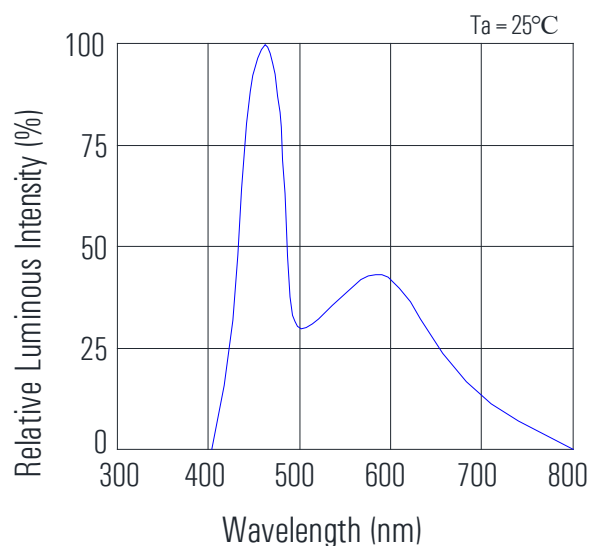
Relative Luminous Intensity Vs Wavelength
