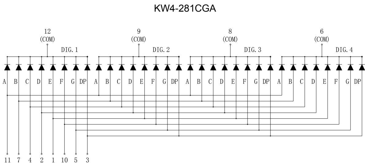
Internal Circuit Diagram (Common Cathode)
