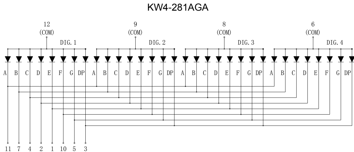
Internal Circuit Diagram (Common Anode)
