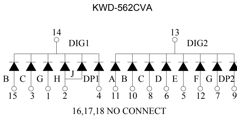
Internal Circuit Diagram (Common Cathode)
