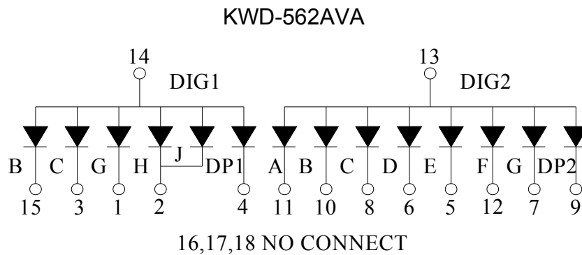
Internal Circuit Diagram (Common Anode)
