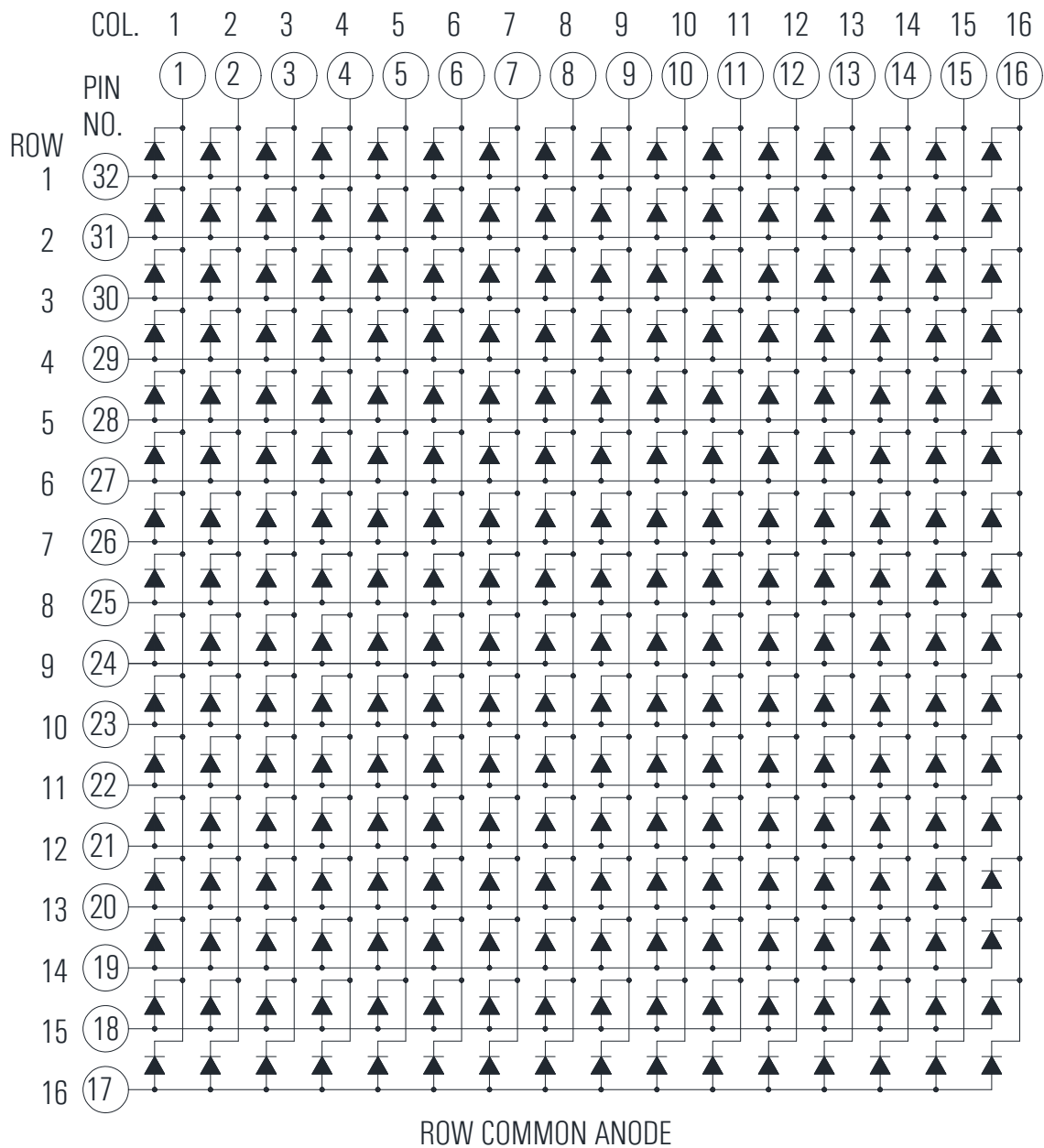
Common Row Anode: KWM-2016162ABB
