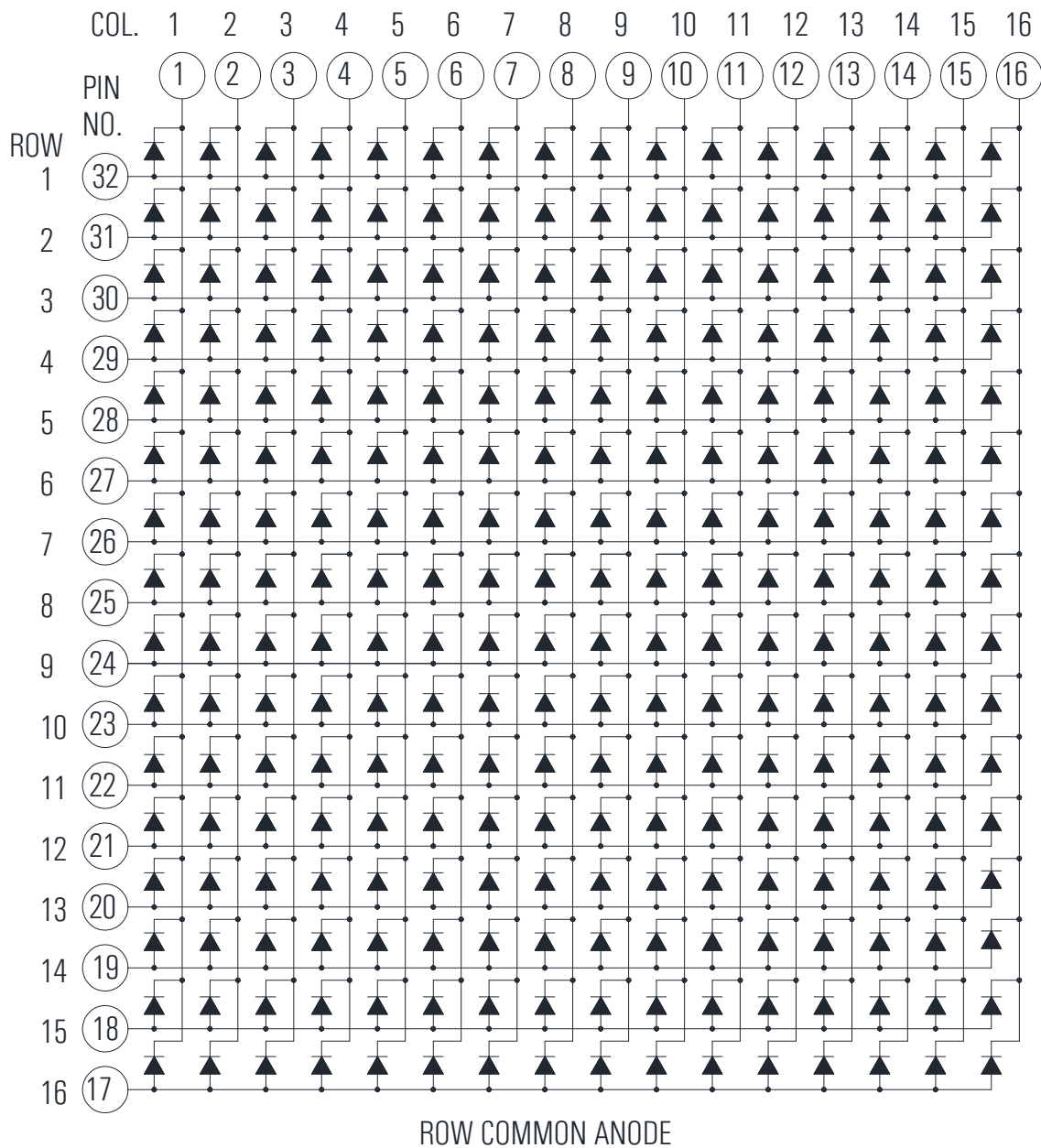
Common Row Anode: KWM-2016162AYB
