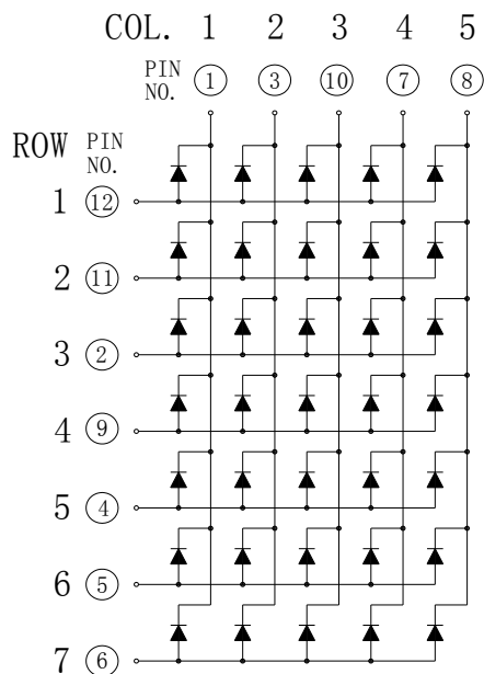
Common Row Anode: KWM-20571AAA
