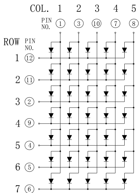
Common Row Cathode: KWM-20571CVA
