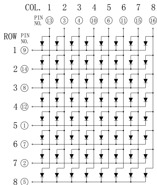
Common Row Cathode: KWM-20881CGA
