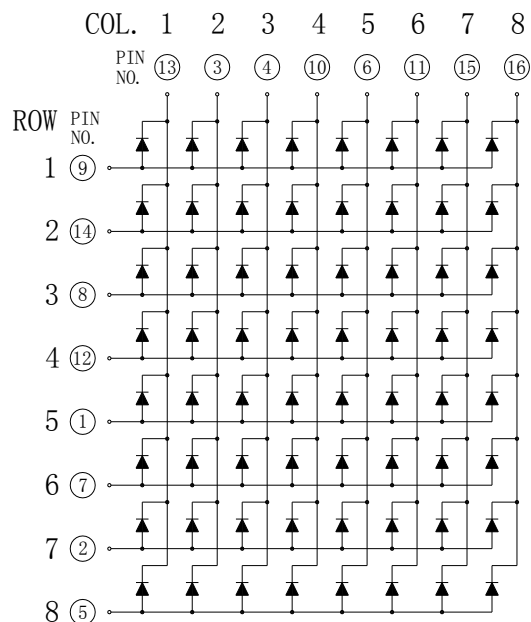
Common Row Anode: KWM-20881AGA
