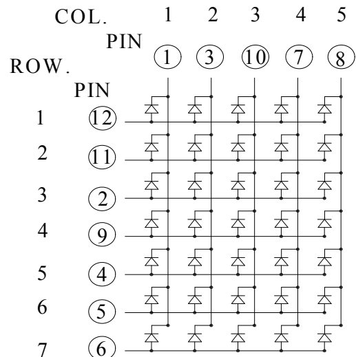
Common Row Anode: KWM-44571AWB
