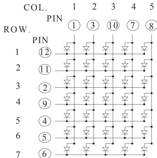
Common Row Cathode: KWM-44571CWB
