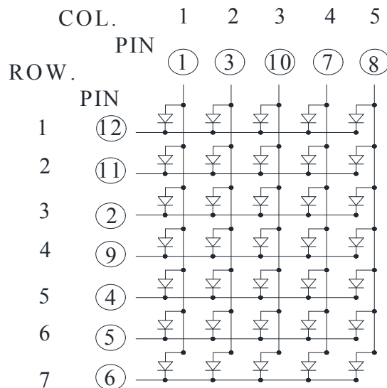
Common Row Cathode: KWM-44571CAB
