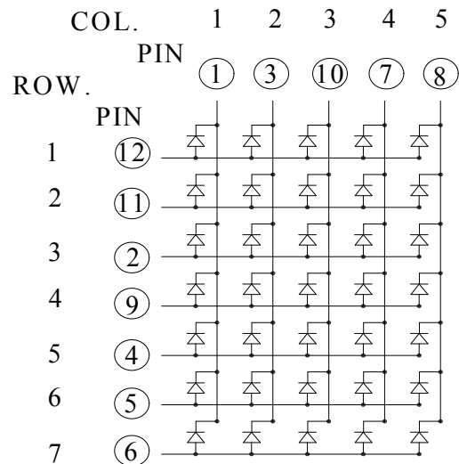
Common Row Anode: KWM-44571AAB
