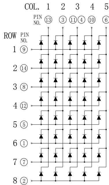
Common Row Anode: KWM-50581AVB
