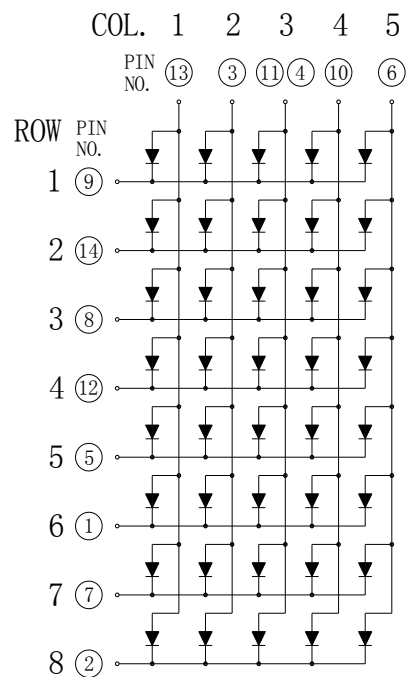
Common Row Cathode: KWM-50581CVB
