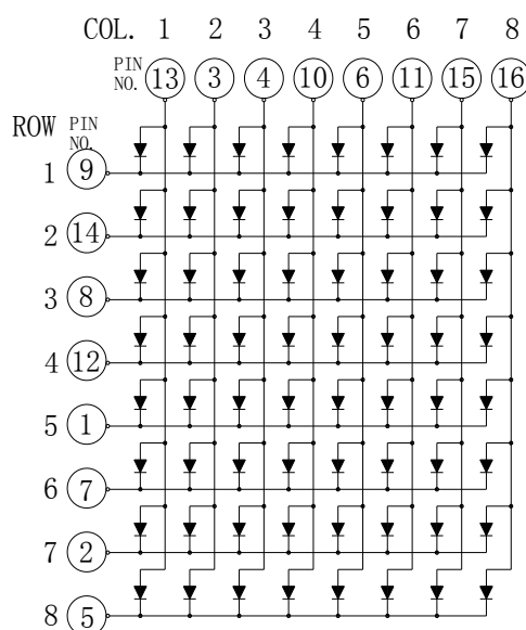
Common Row Cathode: KWM-50881CWB
