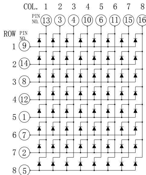
Common Row Cathode: KWM-50881CWB
