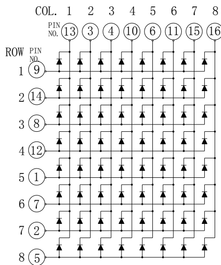
Common Row Anode: KWM-R30881AGB
