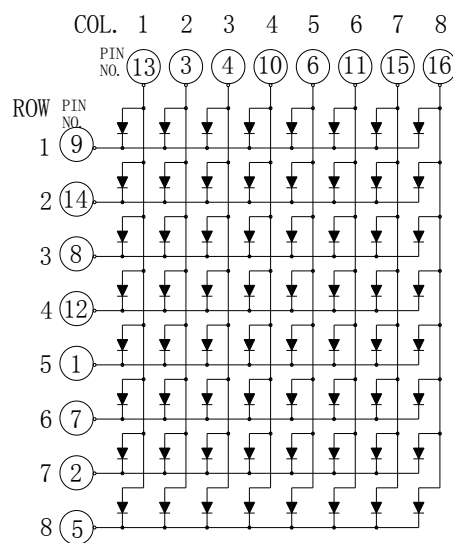
Common Row Cathode: KWM-R30881CGB
