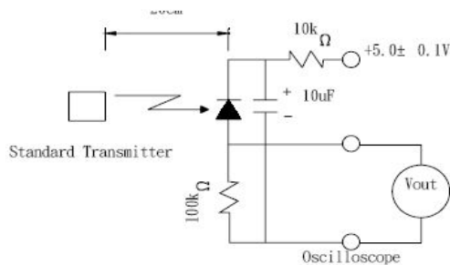
Fig.-2 Measuring Method
