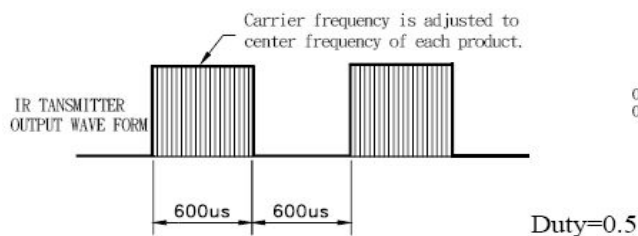
Fig.-1 Transmitter Wave Form
