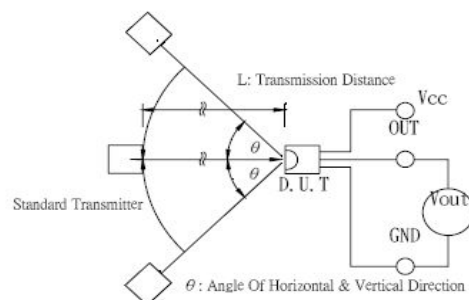
Fig.-3 Measuring System
